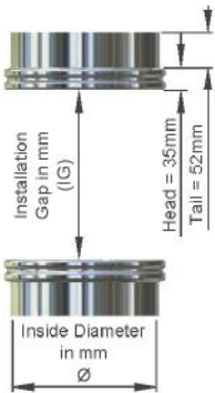
In-line static equipment IG = CL - 10mm (Minimum)
