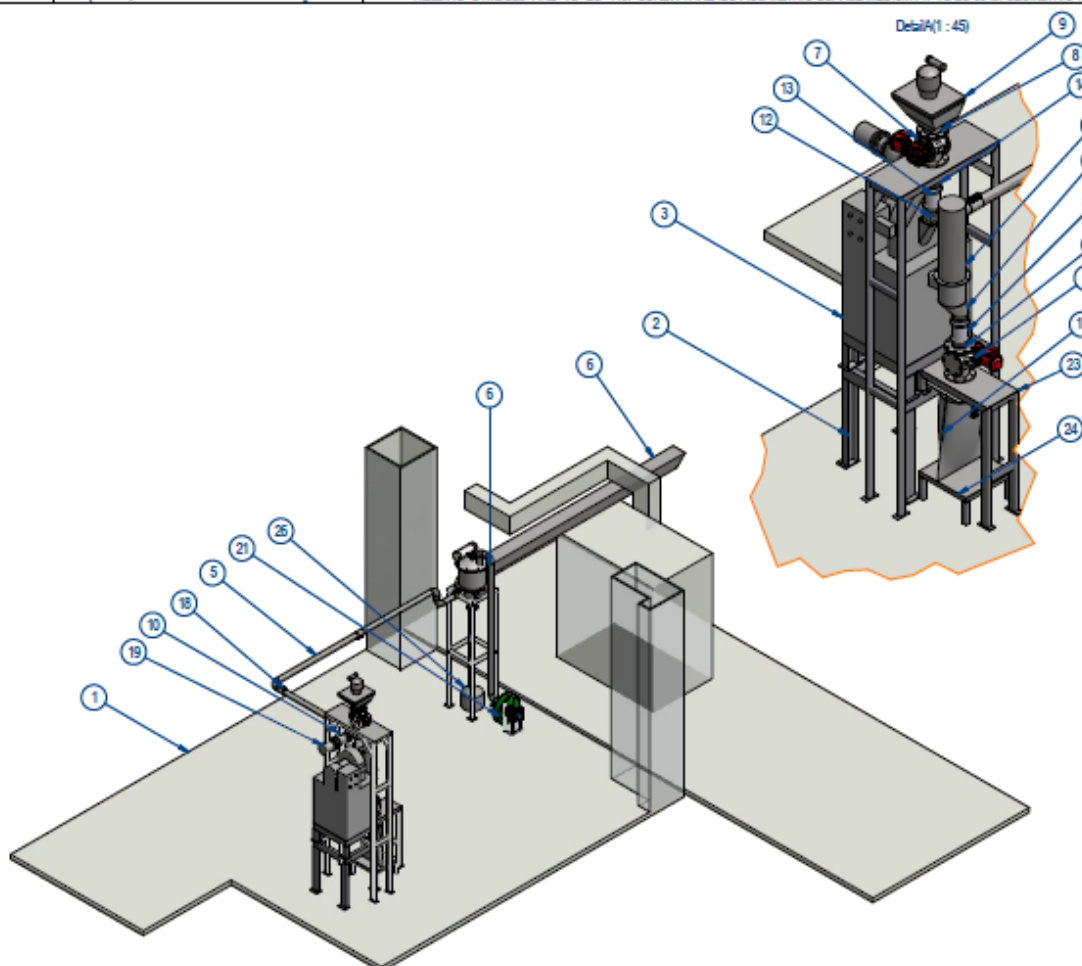
Isometric View 01 (1 : 90)
