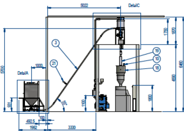
Overview Drawing (1 : 100)
